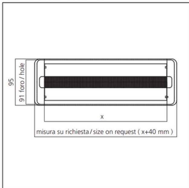
sez. incassato chiuso / embedded section closed
